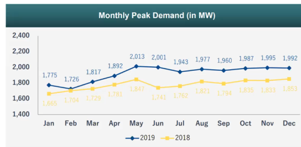
Figure 11. 2018 vs. 2019 Peak Demand, Mindanao
